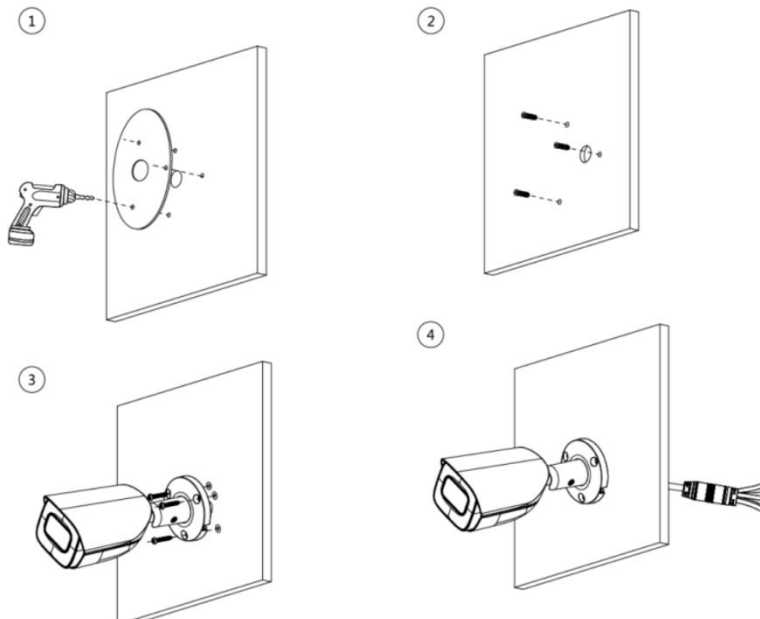
Figure 3-7 Cable going through the mounting surface
