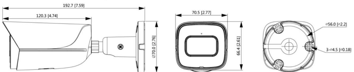
Figure 3-2 Dimensions (mm [inch])
